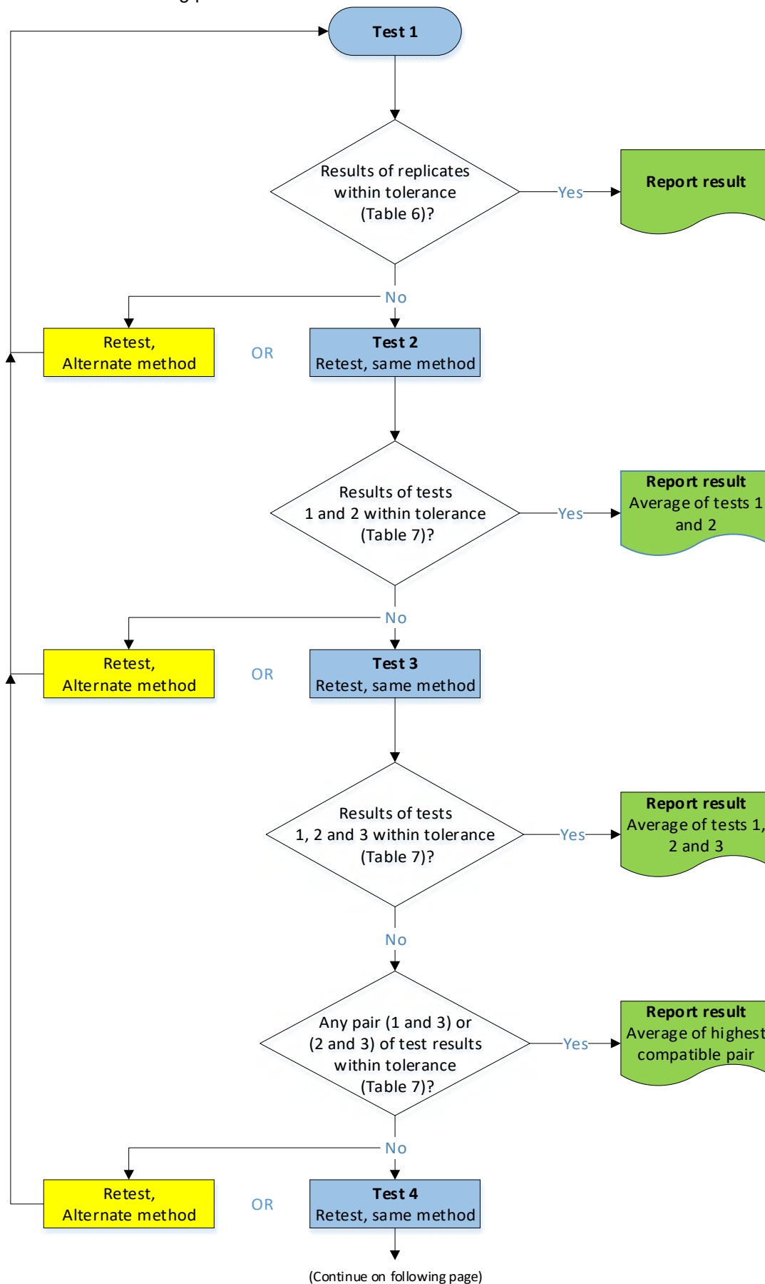
Flow chart of the retesting procedure to obtain in-tolerance results
